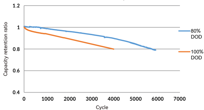
12V460Ah different DOD 0.2C cycle life curve @RT
