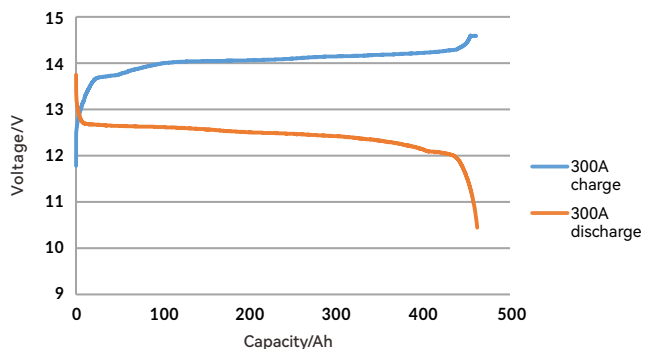
12V460Ah Charge-discharge capacity curve@RT
