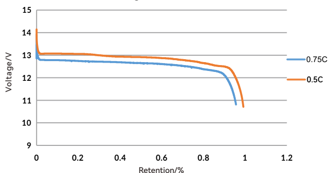
12V460Ah Discharge curve at different rates@RT
