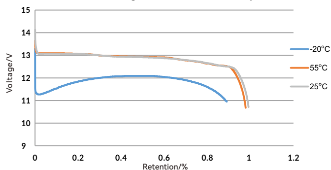
12V460Ah discharge curve at different temperatures
